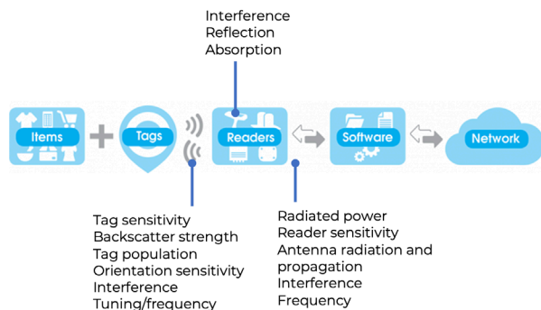
Figure 1: RAIN RFID System Overview
