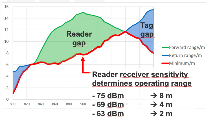
Figure 8: RAIN RFID System limitations
