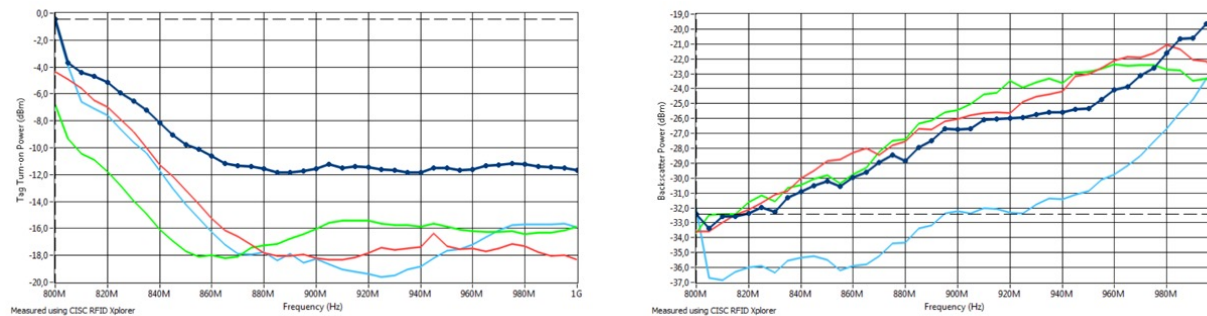
Figure 6: P_{tag,read} and P_{tag,back} example A
