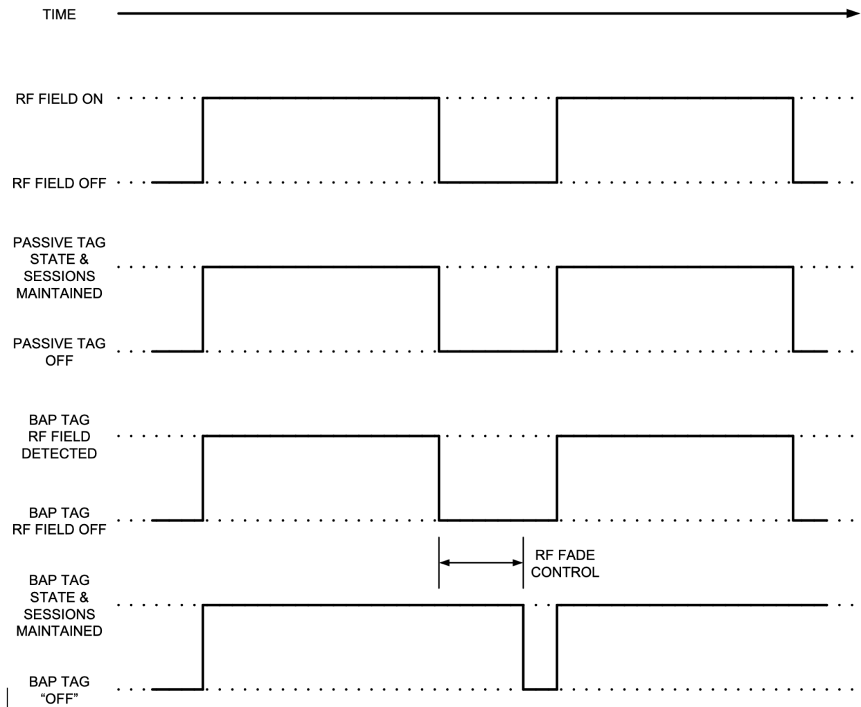
Figure 3: RF Fade control
