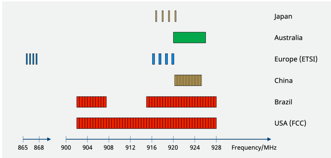
Figure 2: Global RAIN RFID radio bands overview
