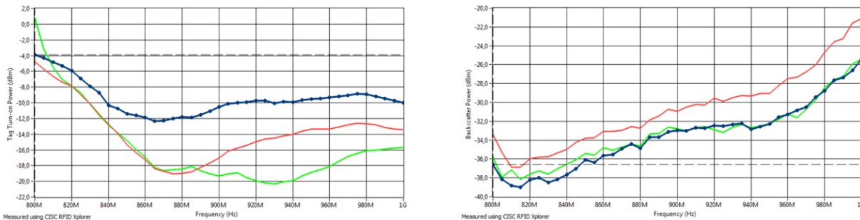
Figure 5: P_{tag,read} and P_{tag,back} example A
